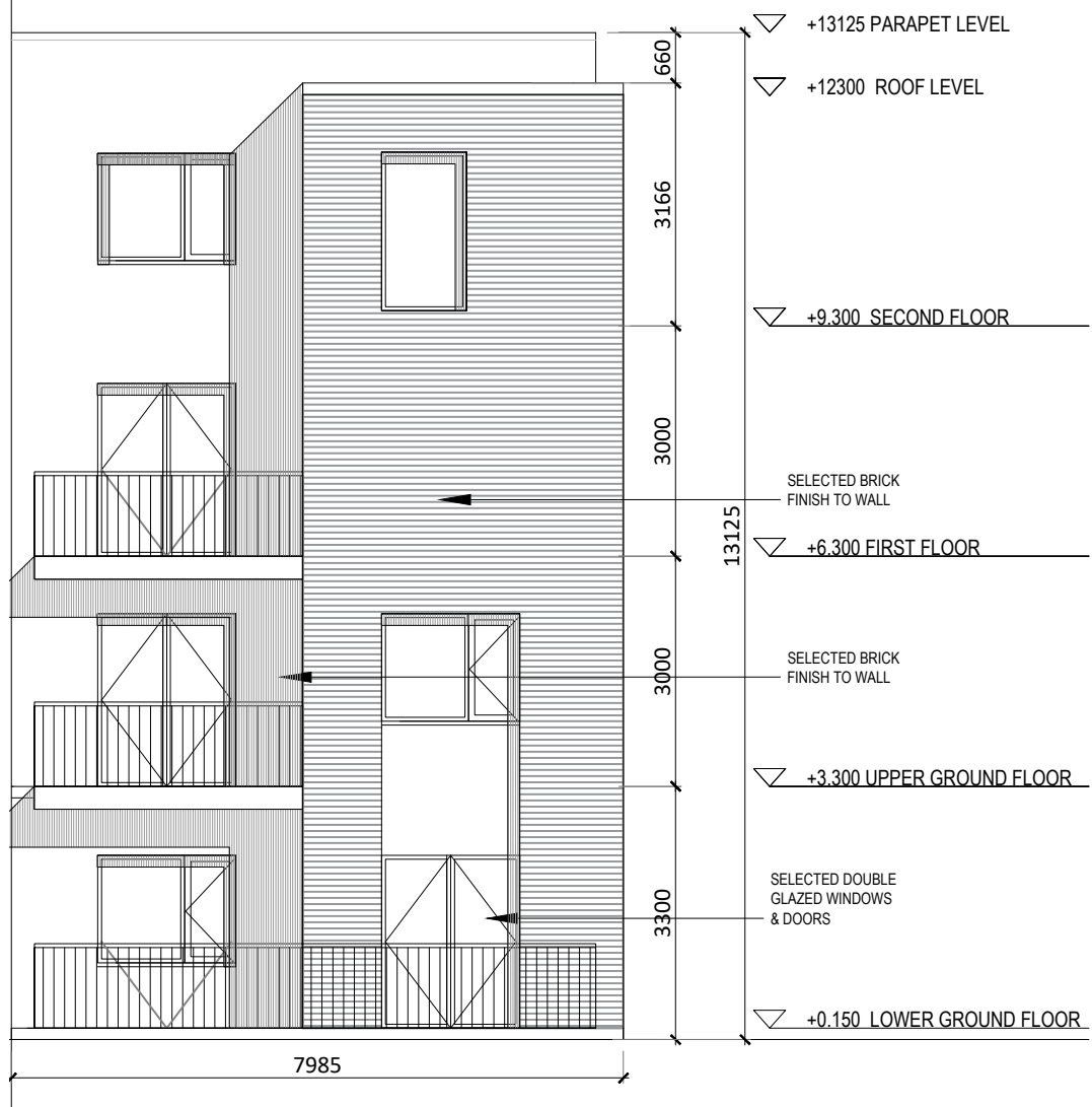
North Elevation to Park 1:100
