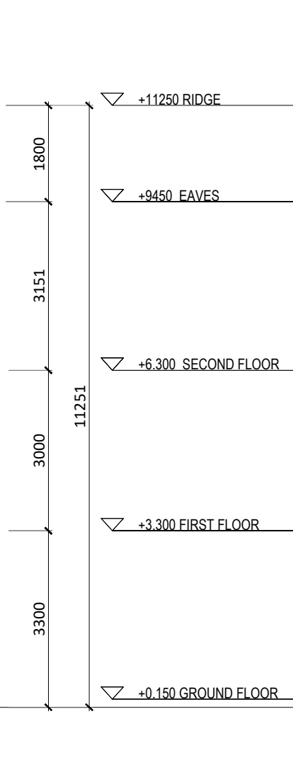
Front Elevation 1:100
