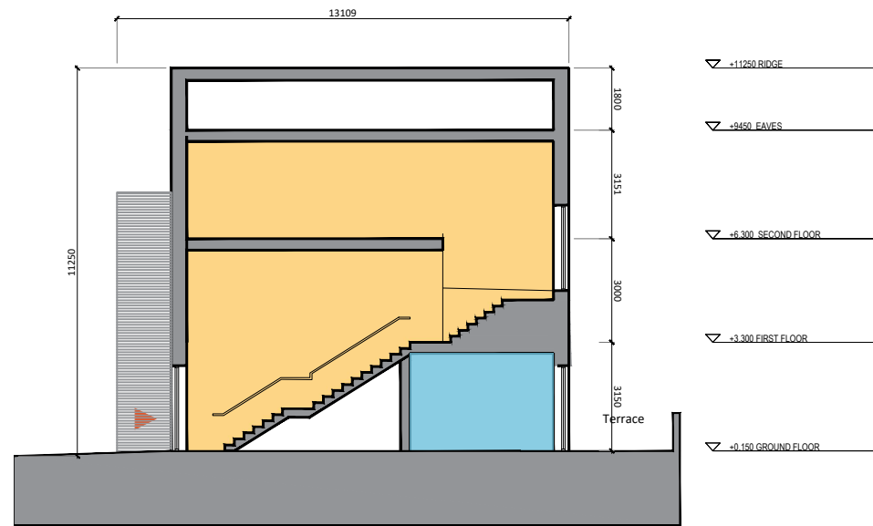
Section 1:200
