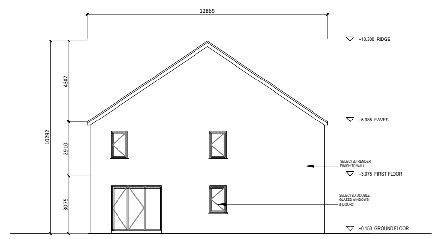
Side Elevation 1:200
