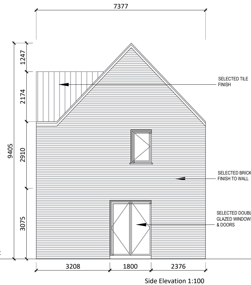
Side Elevation 1:100
