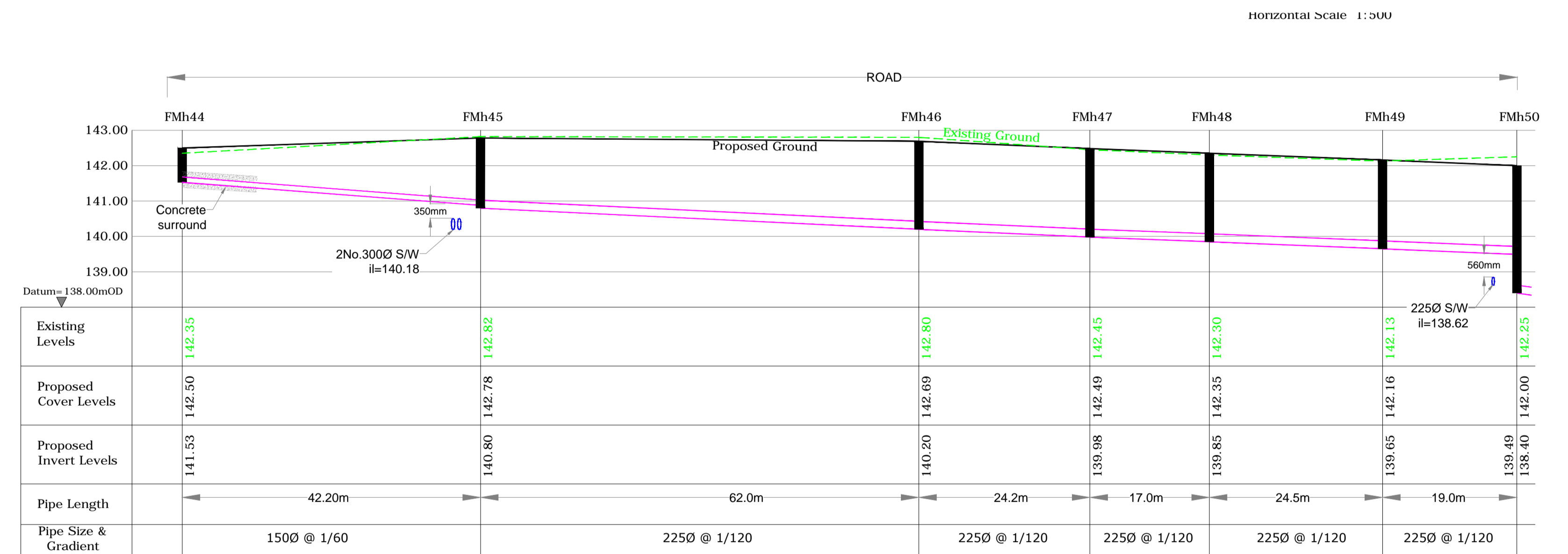
Foul Longitudinal Section FMh44 to FMh50 Vertical Scale 1:100 Horizontal Scale 1:500
