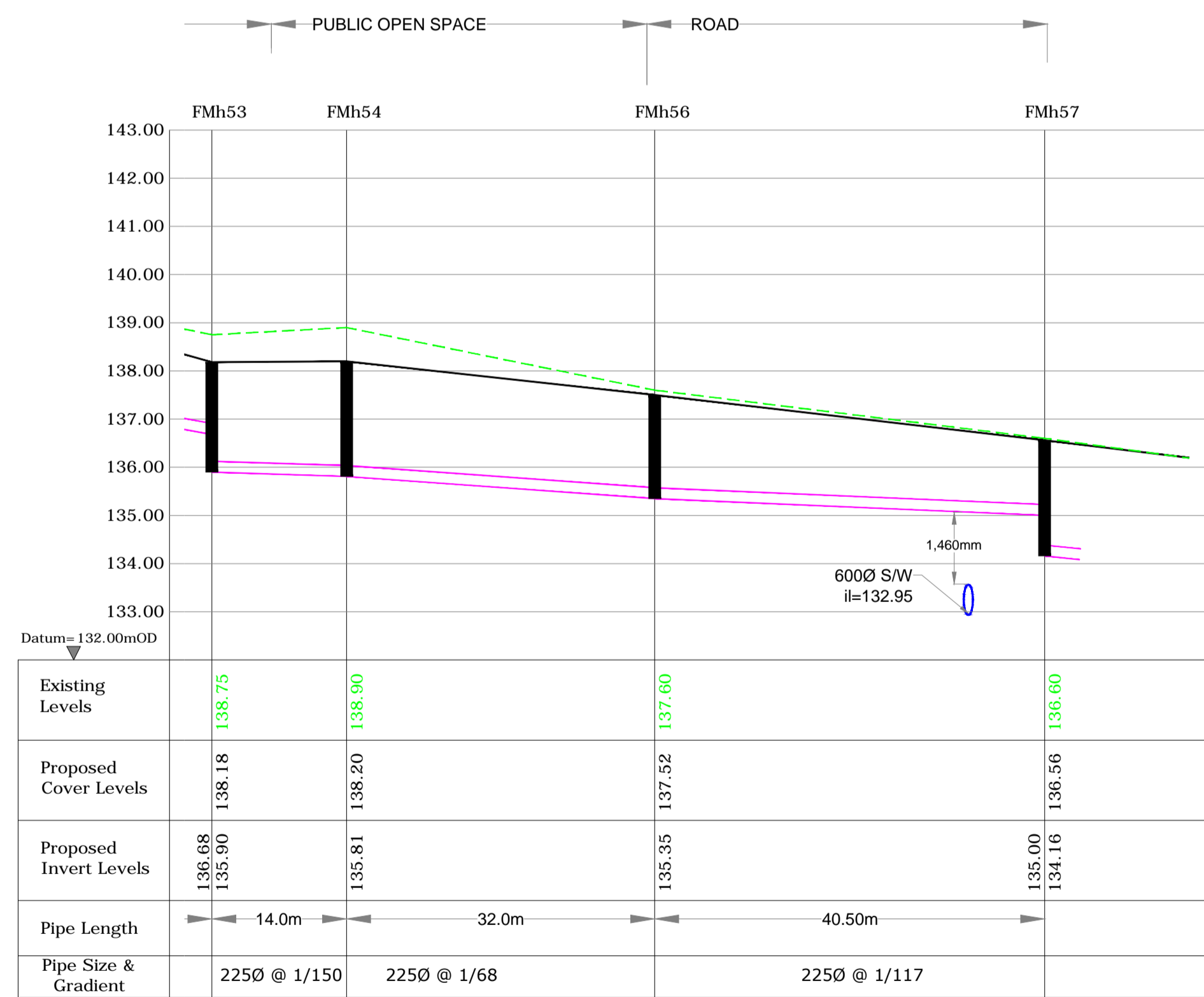
Foul Longitudinal Section FMh53 to FMh57 Vertical Scale 1:100 Horizontal Scale 1:500
