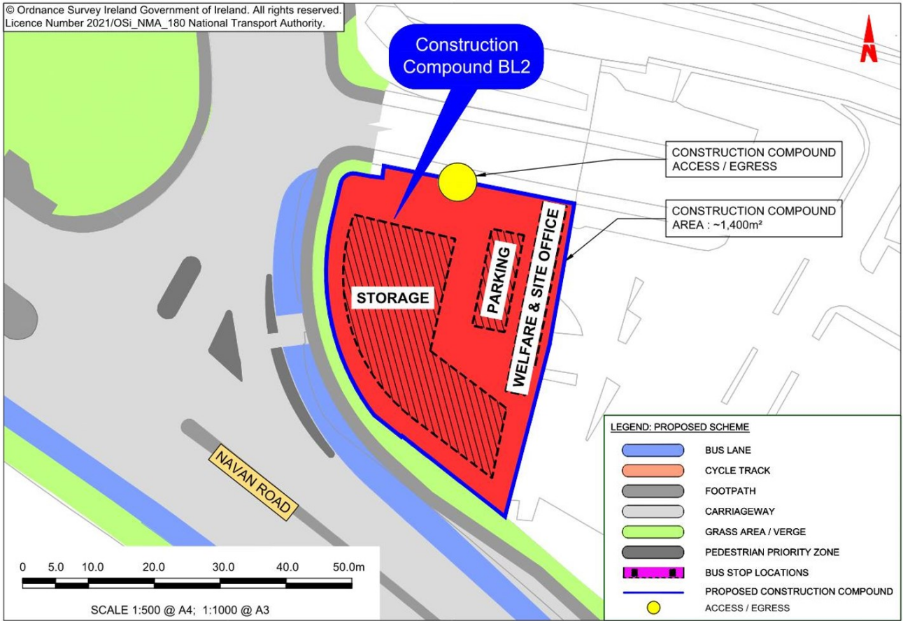
Image 7.2: Layout of Construction Compound BL2
