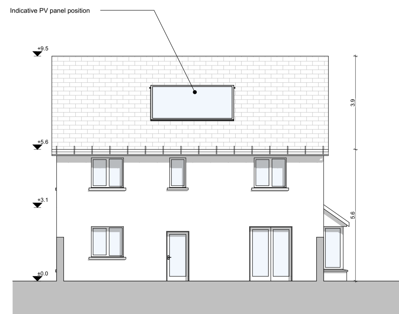
Rear Elevation SCALE 1:100
