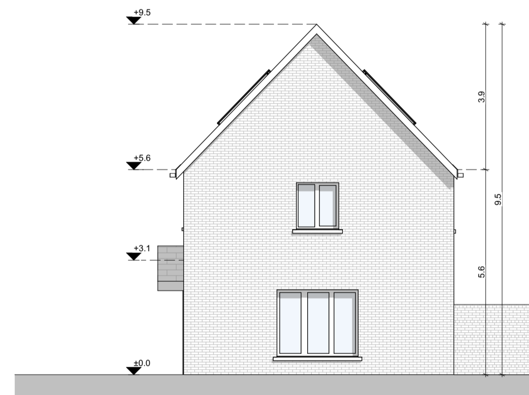
Side Elevation (South) SCALE 1:100
