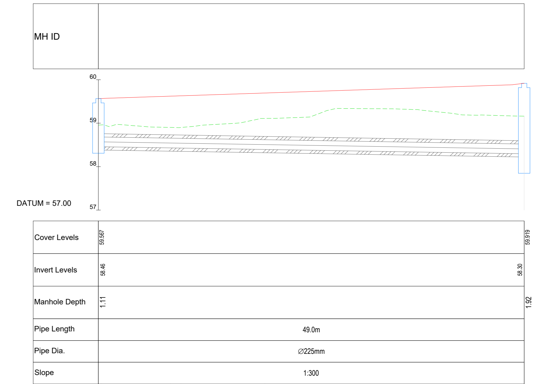
SWMH 6E-0 TO SWMH 6E-2 - PROFILE SCALE: H 1:250, V 1:50
