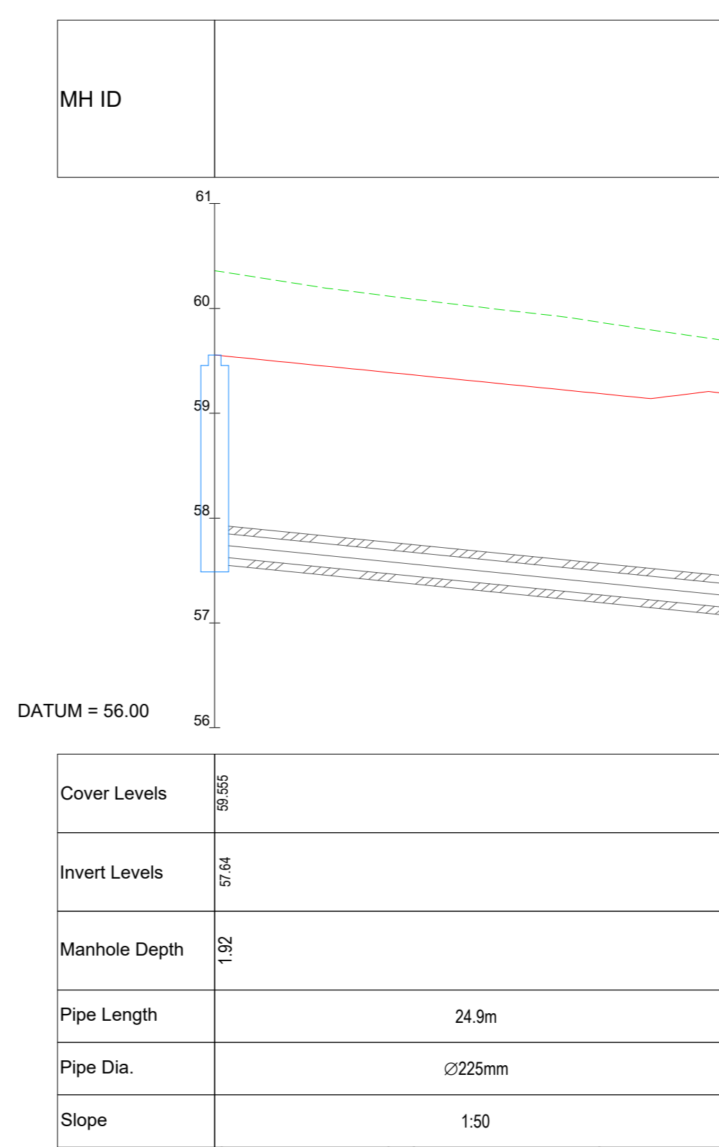
SWMH 8B-0 TO SWMH 8-5 - PROFILE SCALE: H 1:250, V 1:50
