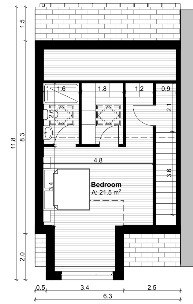
Future Attic Conversion Layout SCALE 1:100
