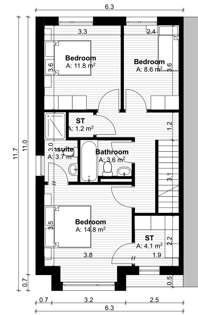
First Floor Plan SCALE 1:100 GFA: 60.9 m²
