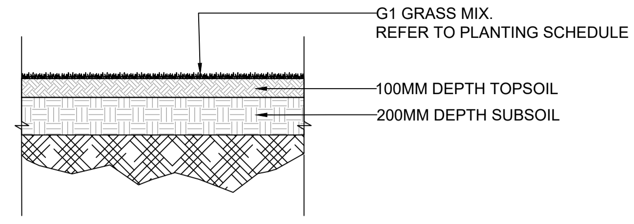
02 TYPICAL GRASS PLANTING 4002 SCALE 1:20 @A1
