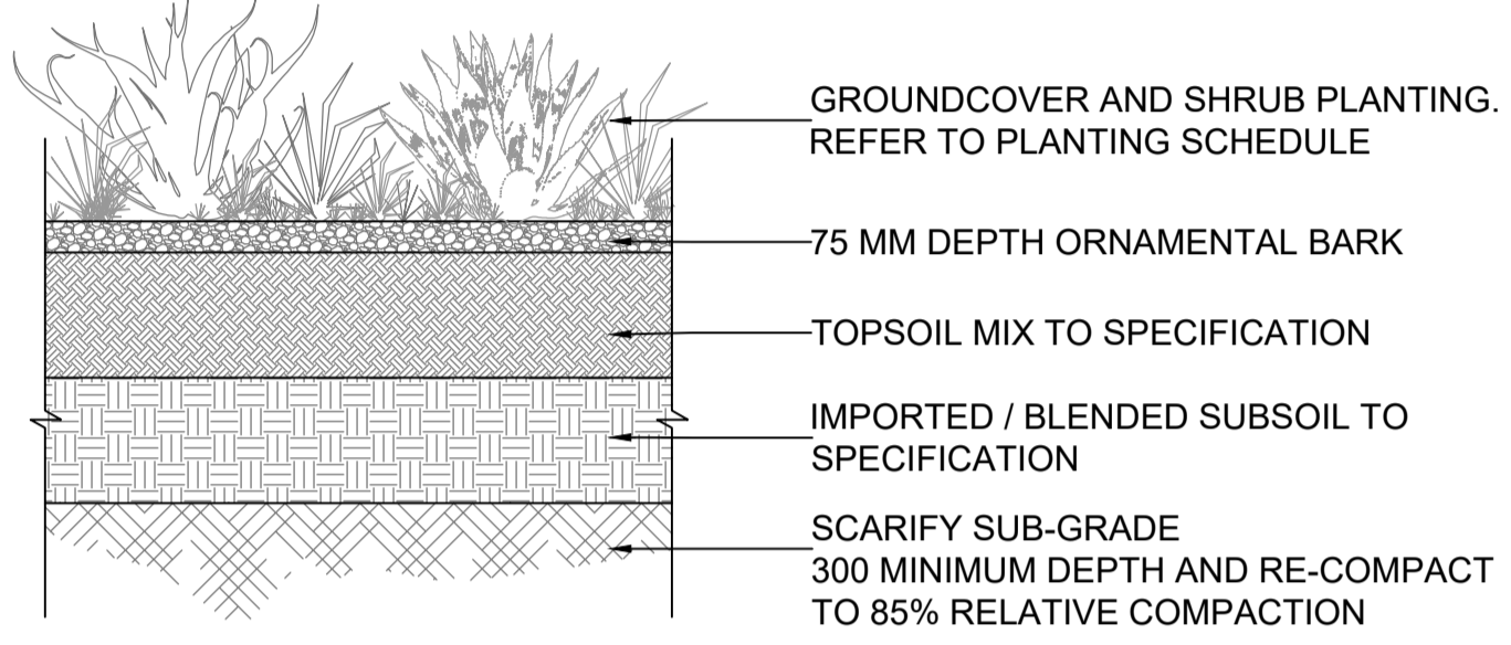
03 TYPICAL SHRUB PLANTING 4002 SCALE 1:20 @A1
