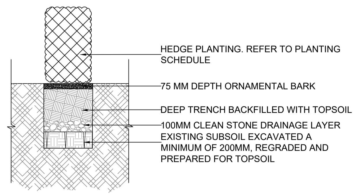
04 TYPICAL HEDGEROW PLANTING 4002 SCALE 1:20 @A1
