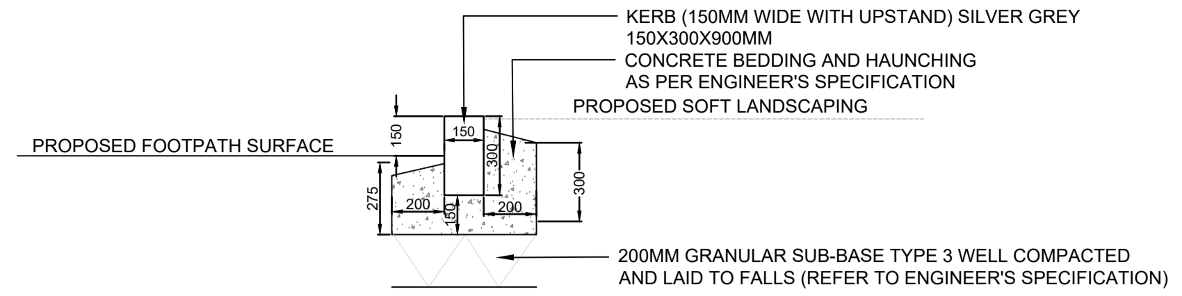
03 TYPICAL DETAIL: KERB WITH UPSTAND (TO SOFT LANDSCAPED AREAS) 4004 SCALE 1:20 @A1
