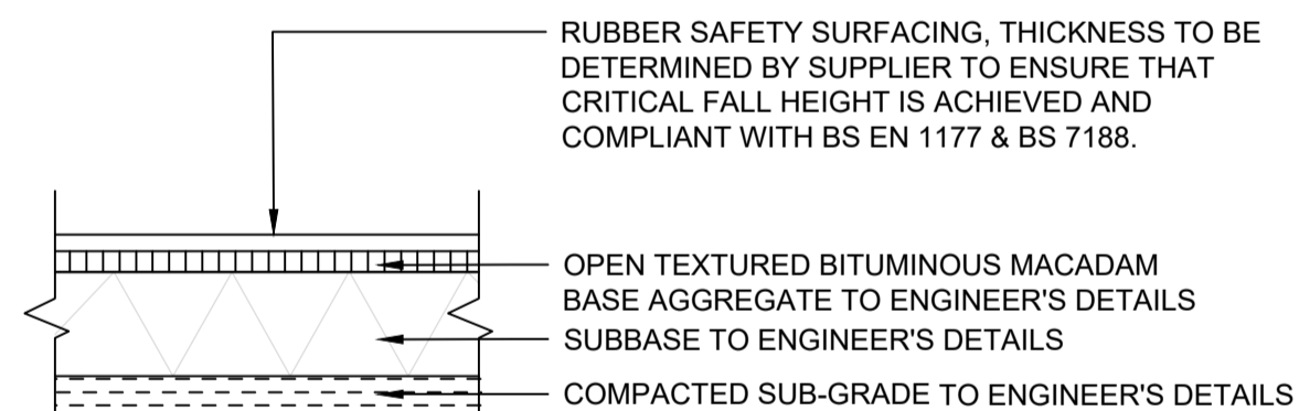
12 TYPICAL DETAIL: SURFACING TO INFORMAL PLAY SPACES 4004 SCALE 1:20 @A1
