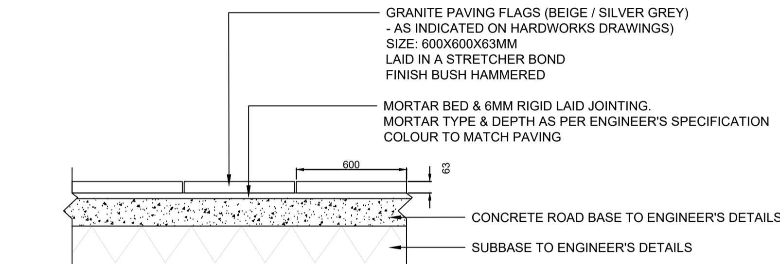
07 TYPICAL DETAIL: HIGH QUALITY PAVING (TYPES A / B) 4004 SCALE 1:20 @A1
