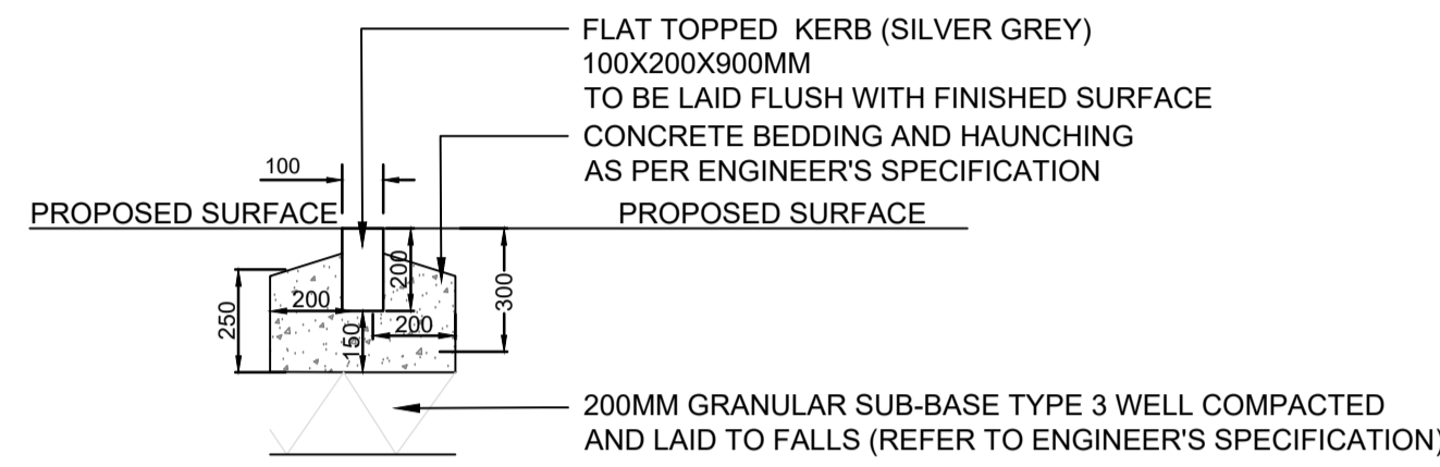
04 TYPICAL DETAIL: FLAT TOPPED KERB (TO SITE BOUNDARY) 4004 SCALE 1:20 @A1
