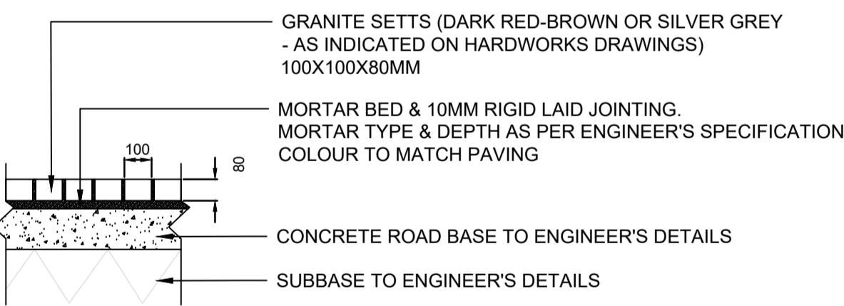
10 TYPICAL DETAIL: PAVING BAND 4004 SCALE 1:20 @A1
