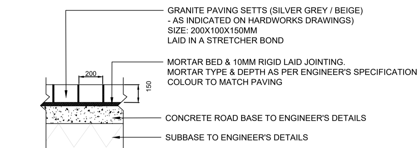
09 TYPICAL DETAIL: HIGH QUALITY PAVING (SHARED SURFACE) 4004 SCALE 1:20 @A1
