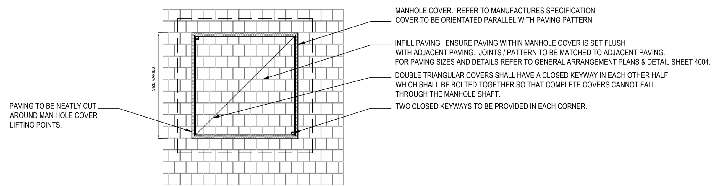
13 TYPICAL DETAIL: RECESSED PAVING COVER 4004 SCALE 1:20 @A1
