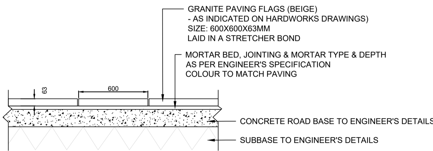
11 TYPICAL DETAIL: PAVING TO FOOTPATHS 4004 SCALE 1:20 @A1
