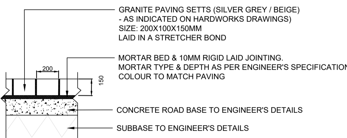
08 TYPICAL DETAIL: HEAVY VEHICLE PAVING (TYPES A / B) 4004 SCALE 1:20 @A1
