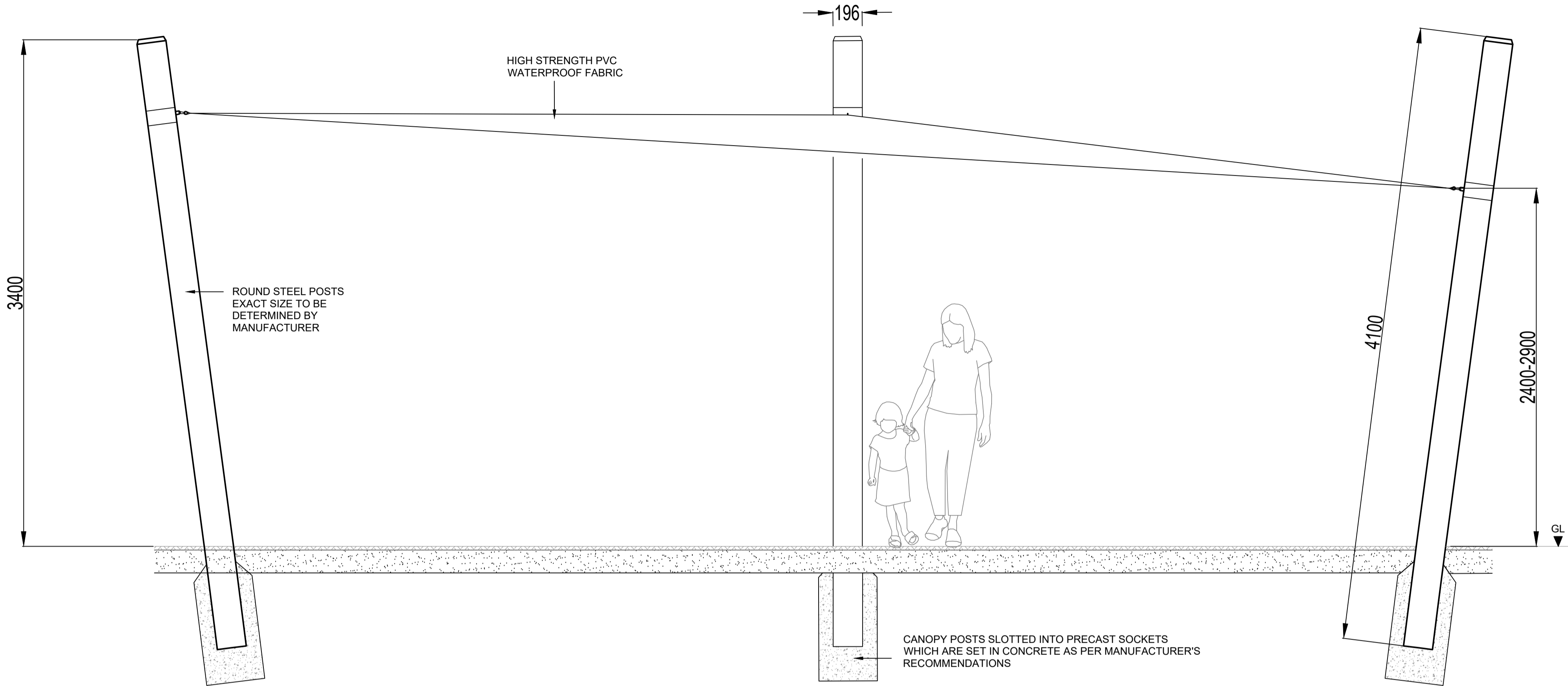
DETAIL REPRESENTING THE DESIGN INTENT FOR THE CANOPY STRUCTURE.
