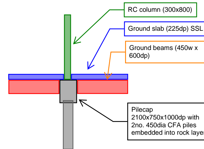
Section Detail
