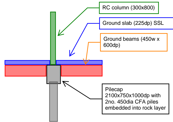
Section Detail
