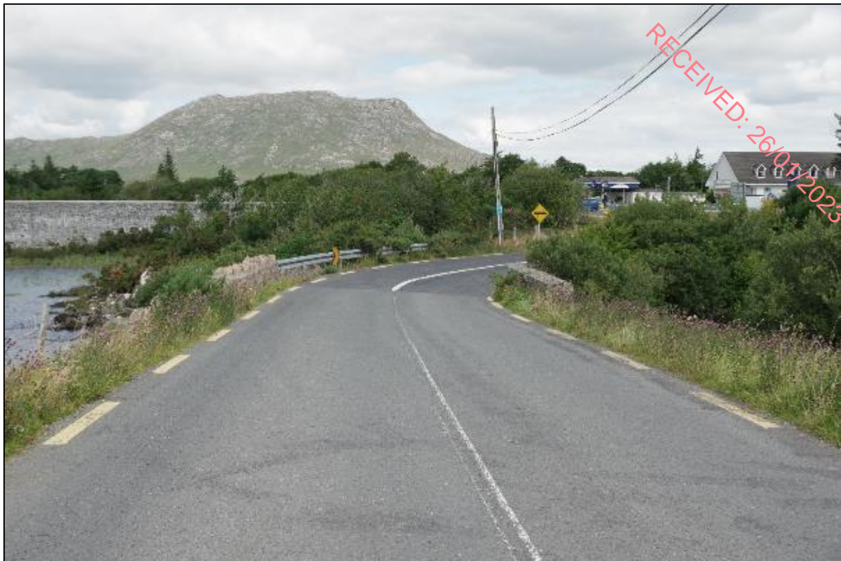
Plate 13.15: Road level view of bridge RPS 3359 on section of grid route to south of Maam Cross taken from south
