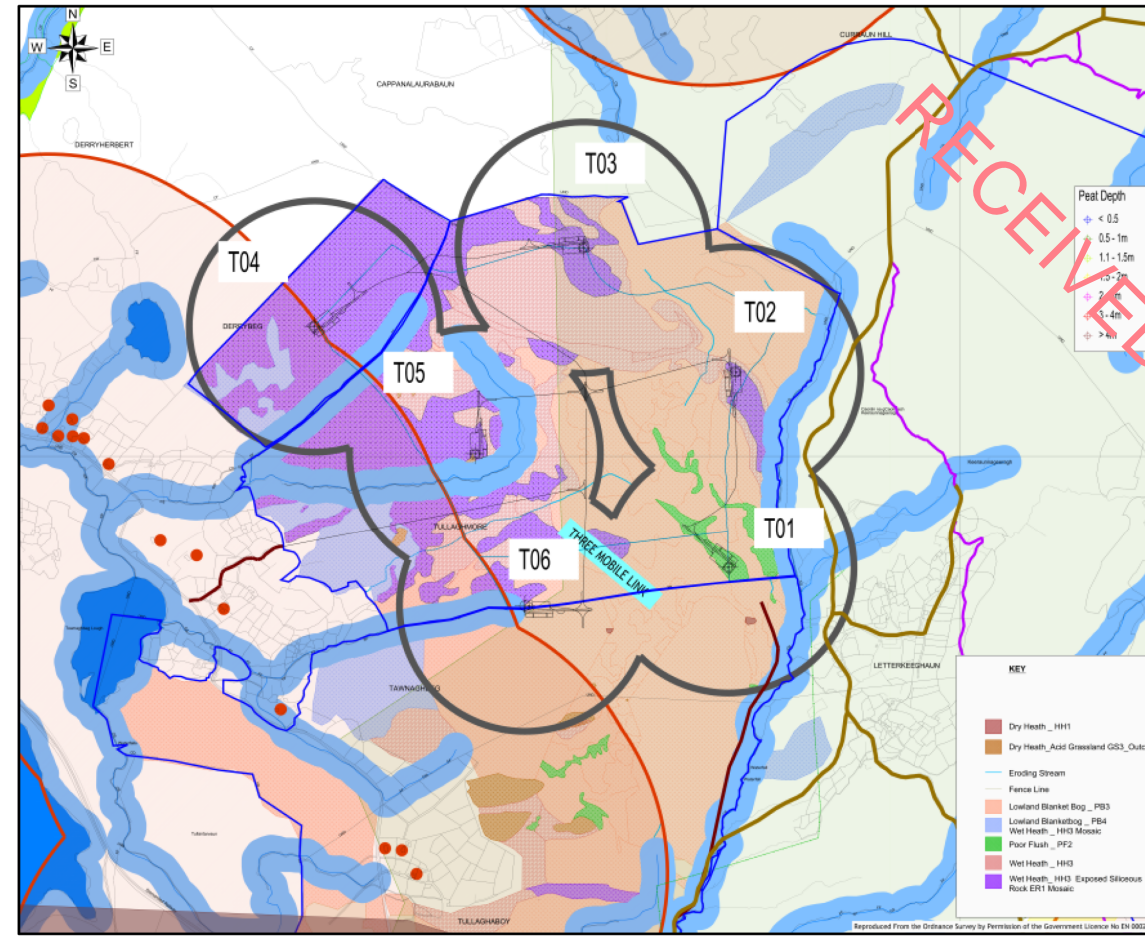
PROPOSED 6 TURBINE LAYOUT 12
