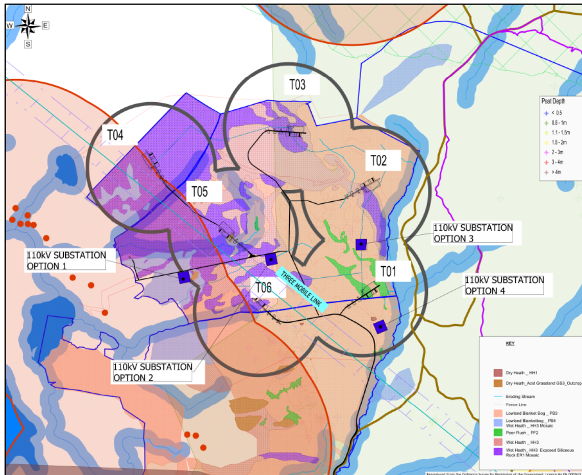
PROPOSED 6 TURBINE LAYOUT 13
