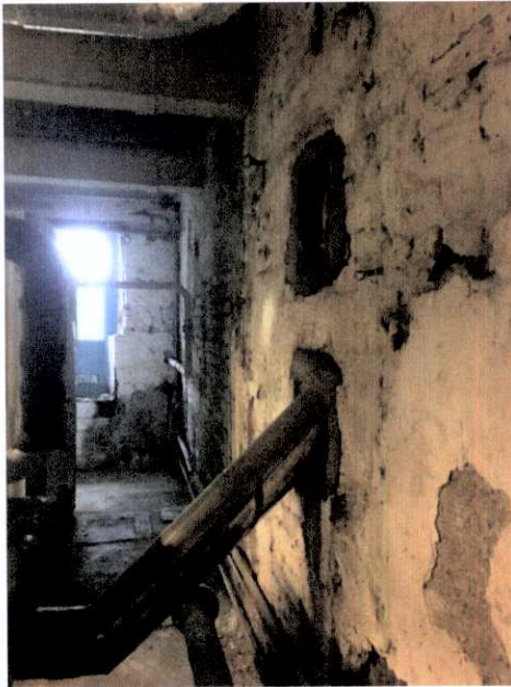
Fig. 33 Former kitchen to northwest at basement level, with original masonry and floor flags evident. Note concrete downstands for concrete floor plate supporting entrance level above.
