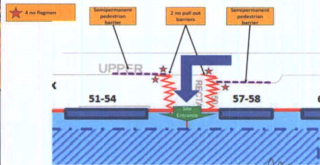
Figure 29. - Typical Pavement Crossover System
