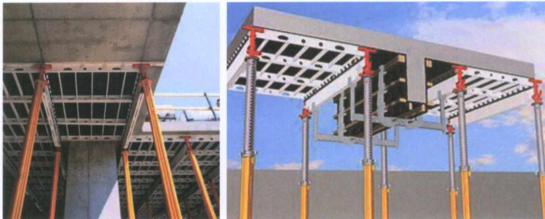
Figure 20 - Typical RC Formwork (Skydeck)
