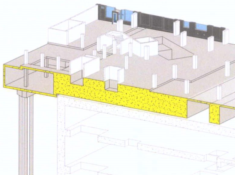
Figure 16. MEW Transfer Slab Detail
