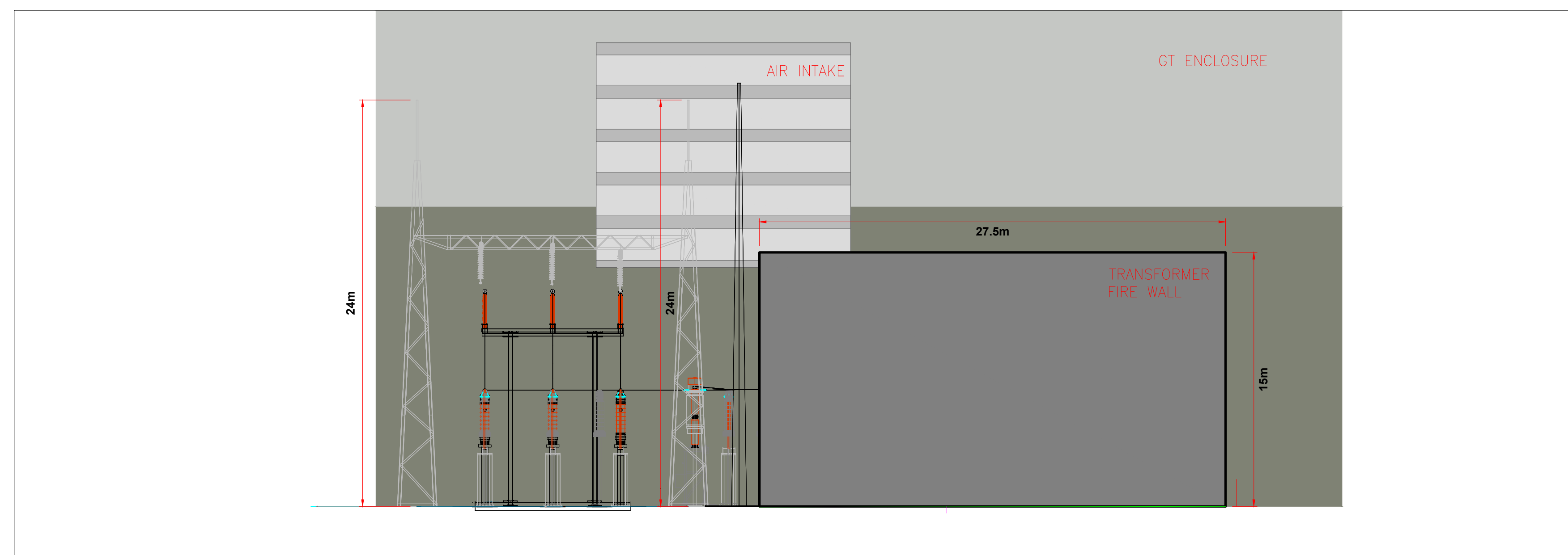
D-D SOUTH WEST ELEVATION 1:200
