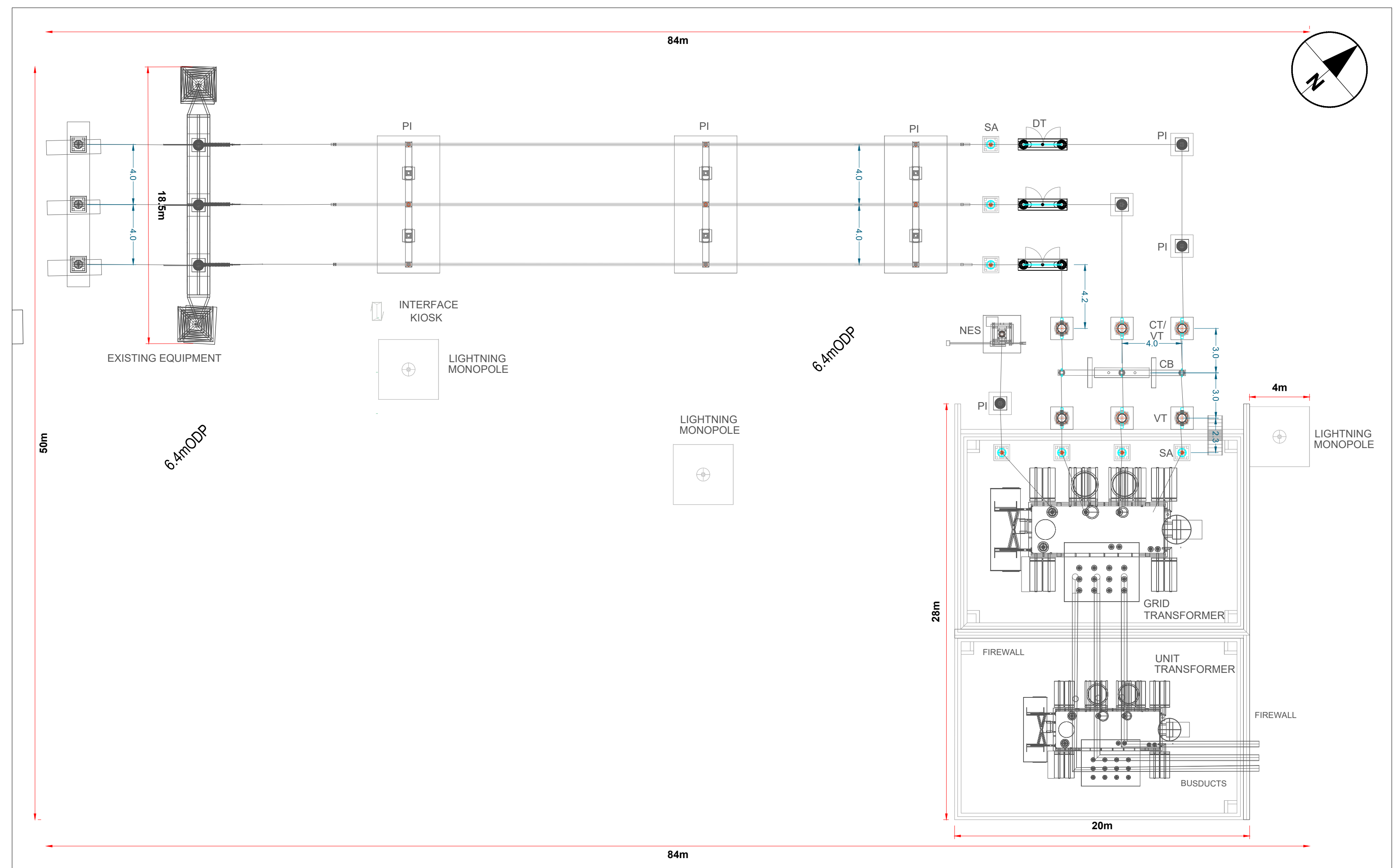
HV Connection & Transformer Plan View Scale 1:200
