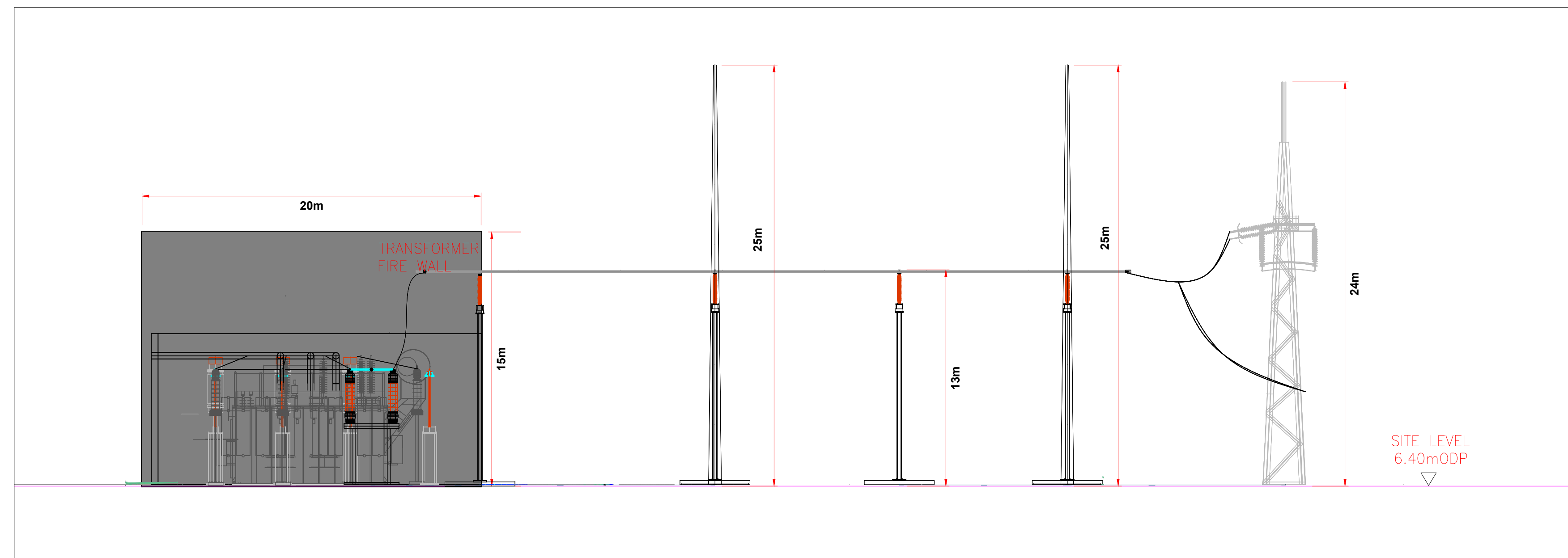
A-A NORTH WEST ELEVATION 1:200
