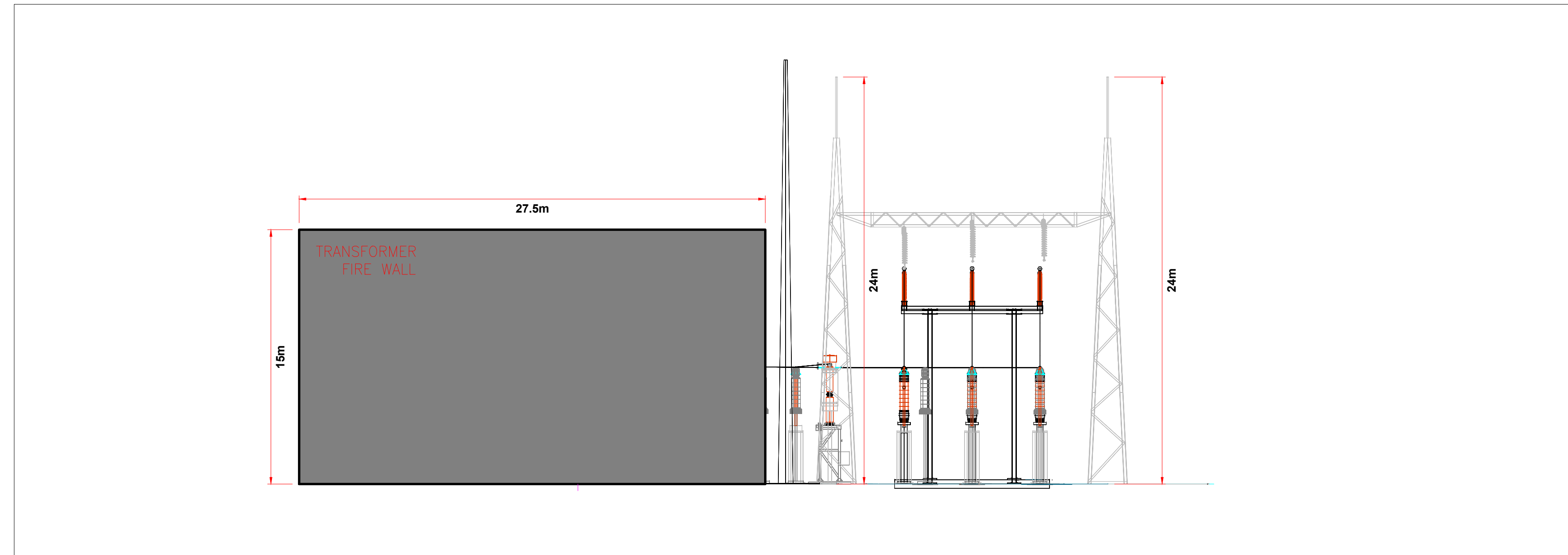
B-B NORTH EAST ELEVATION 1:200
