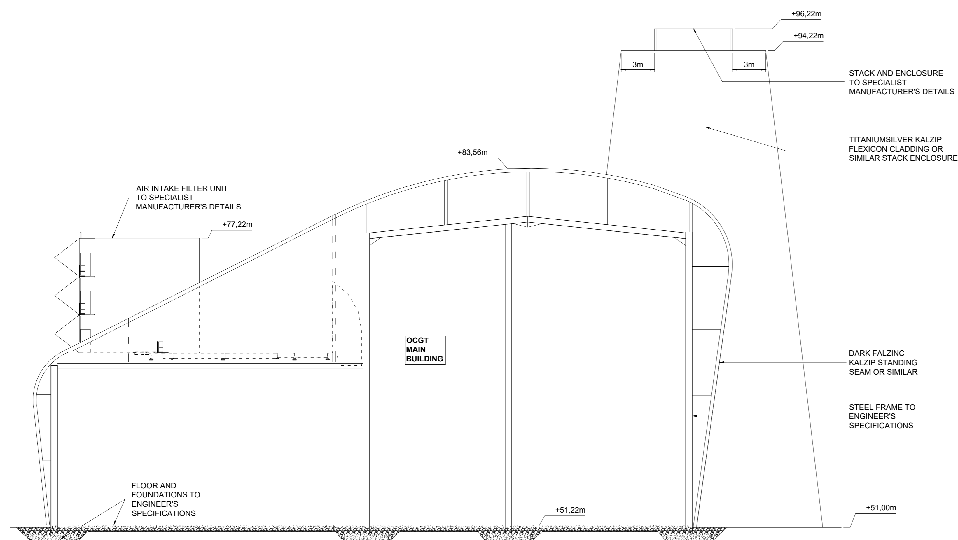
SECTION 1-1 SCALE 1:200
