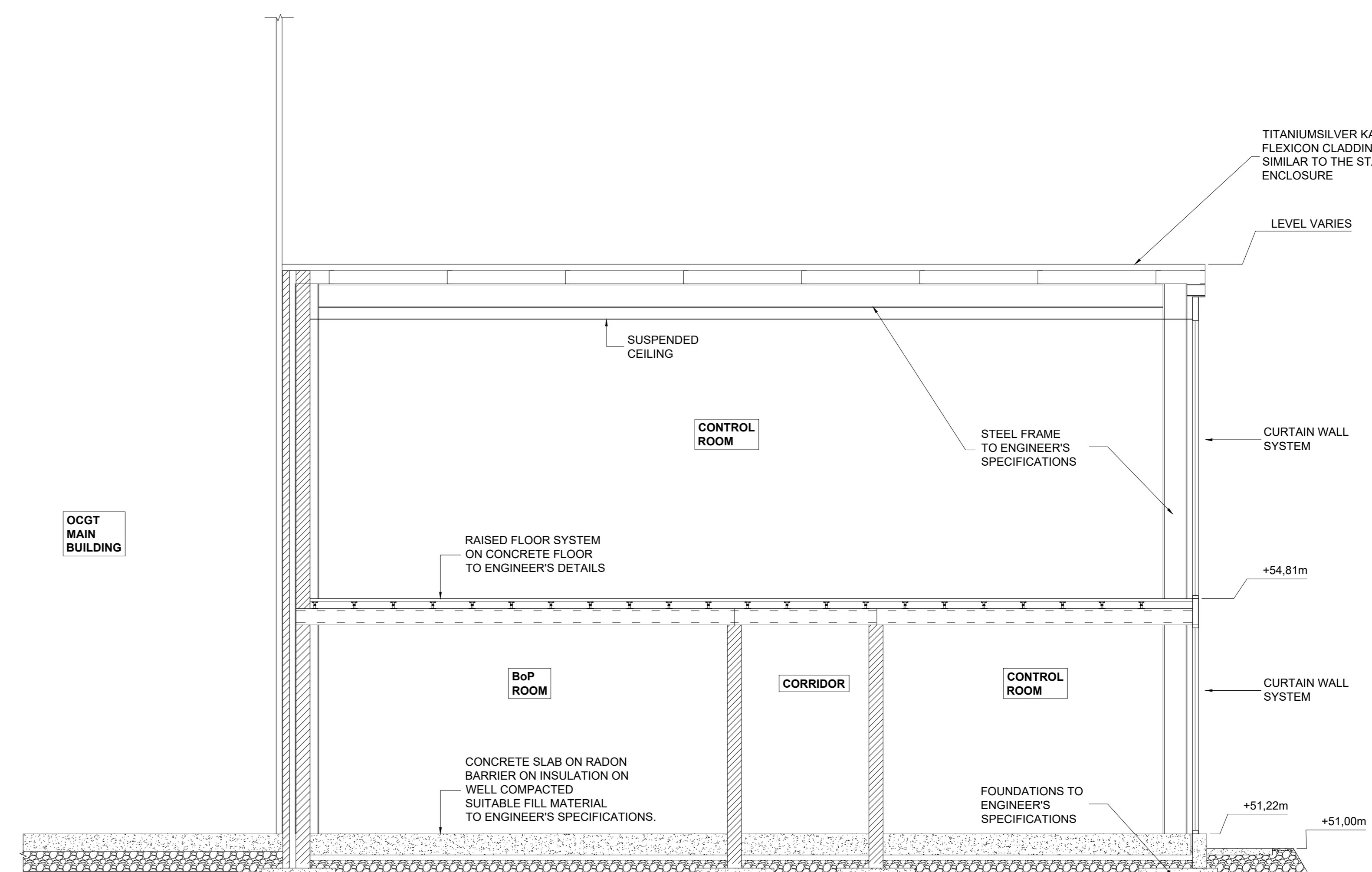
SECTION 2-2 SCALE 1:50
