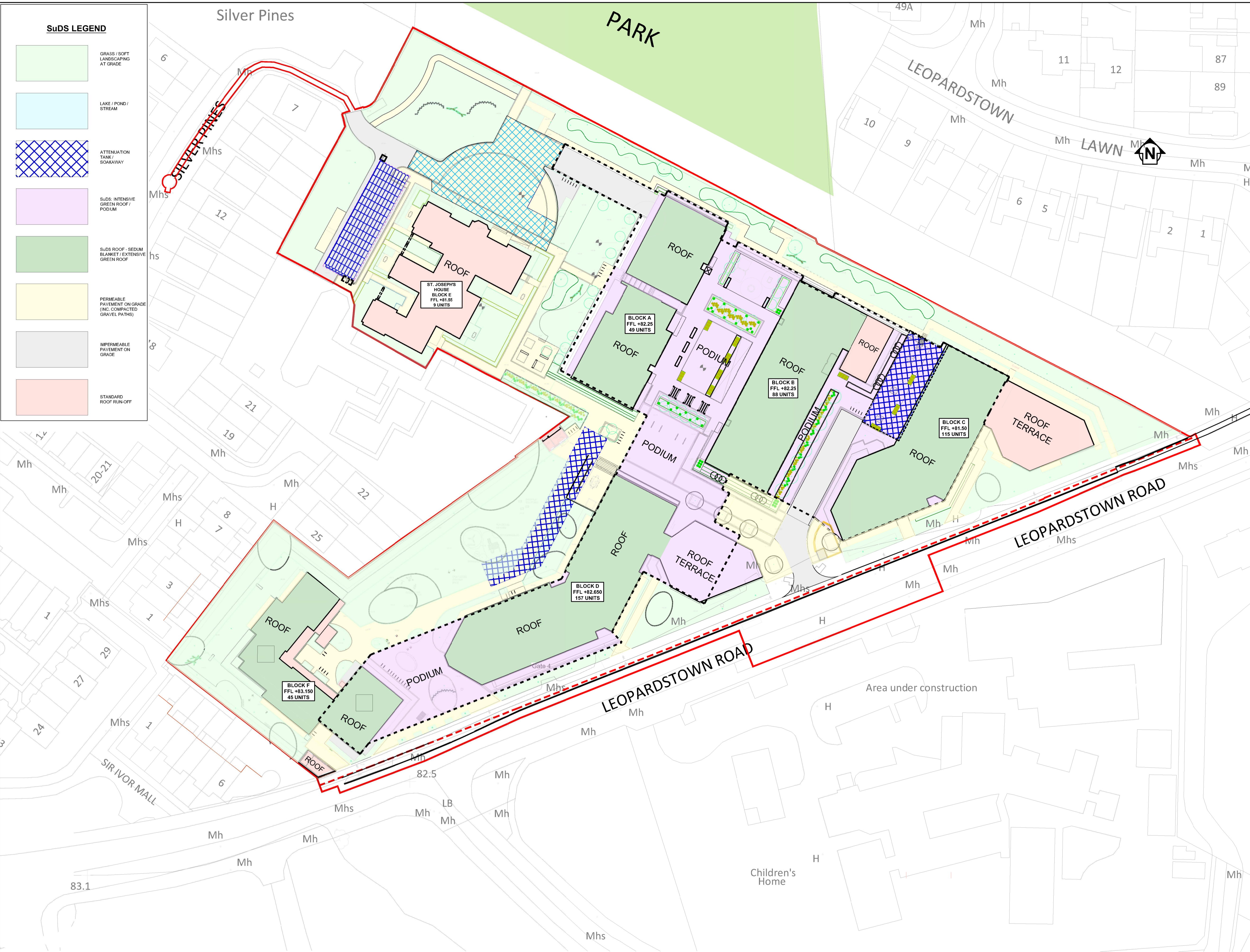
SCHEMATIC SUDS PLAN LAYOUT SCALE @ A1: 1:500 SCALE @ A3: 1:1000
