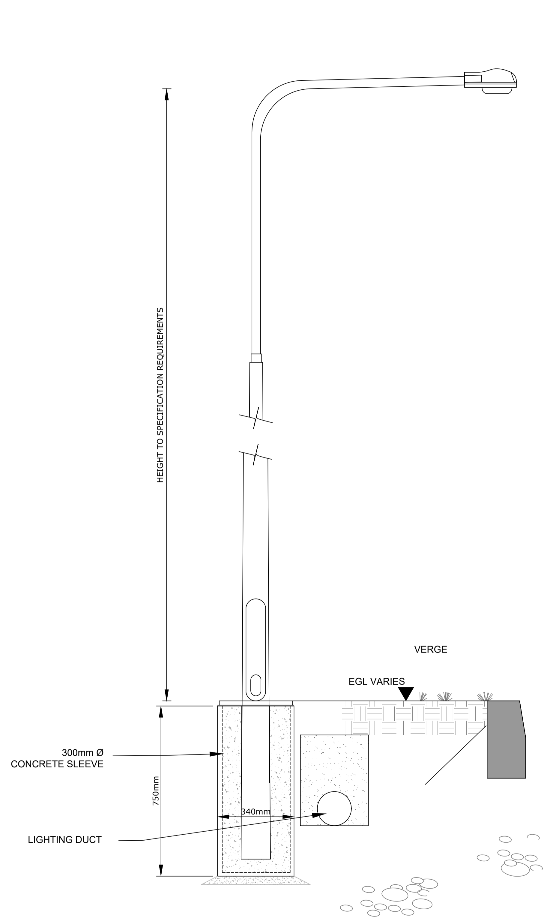
Lighting Column & Surround Detail SCALE 1:10
