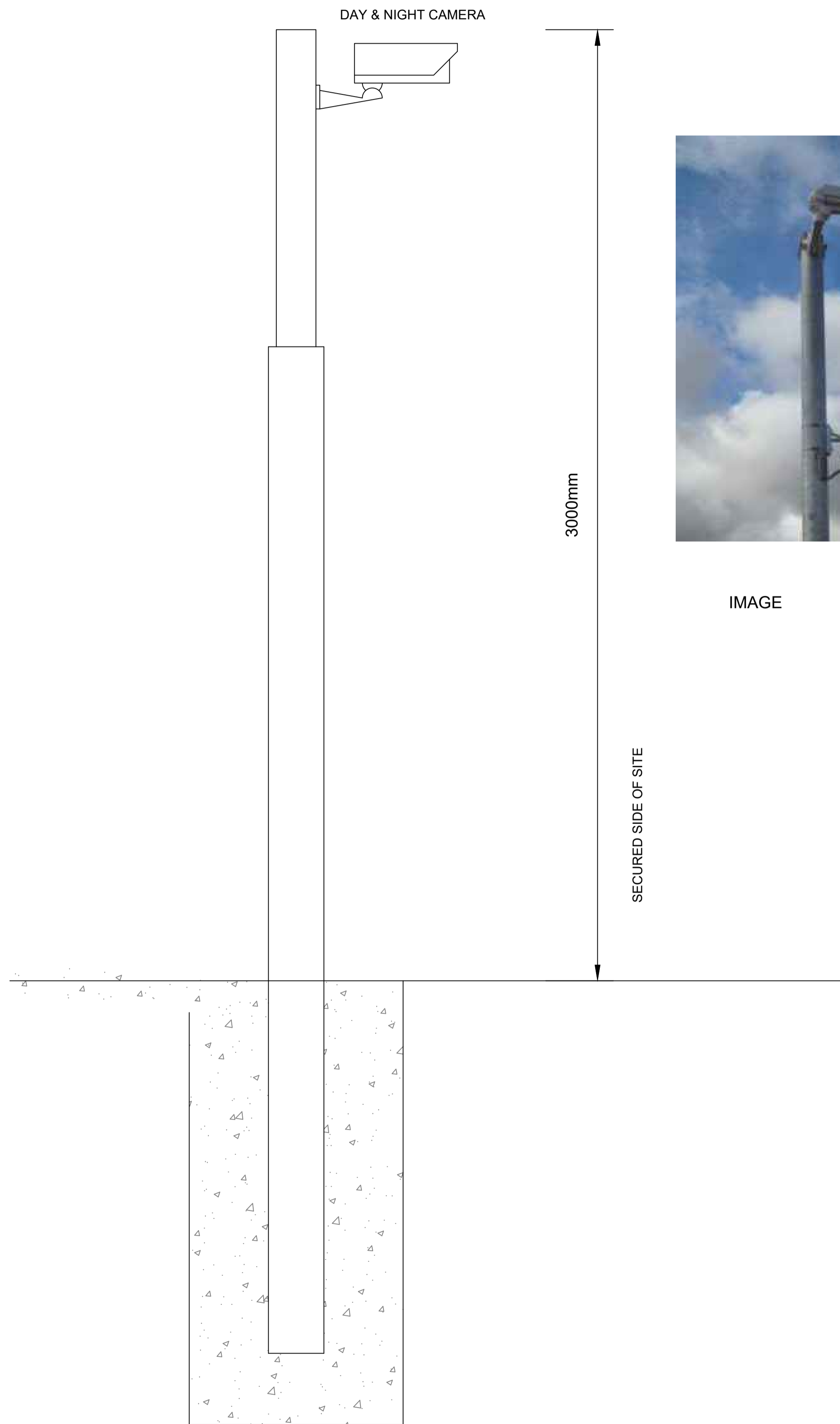
CCTV Camera Column SCALE 1:10
