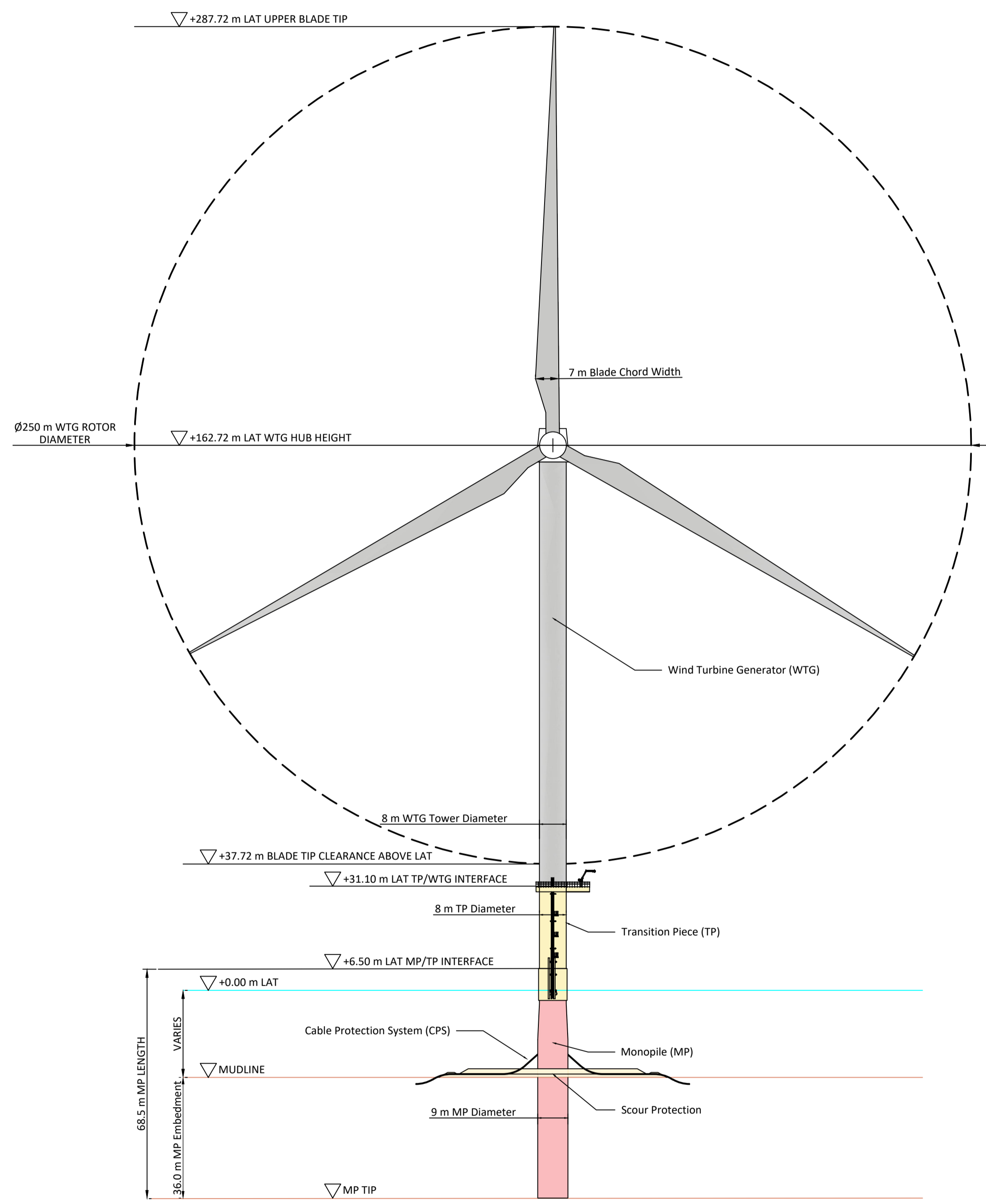
ELEVATION ON MONOPILE ARRANGEMENT
