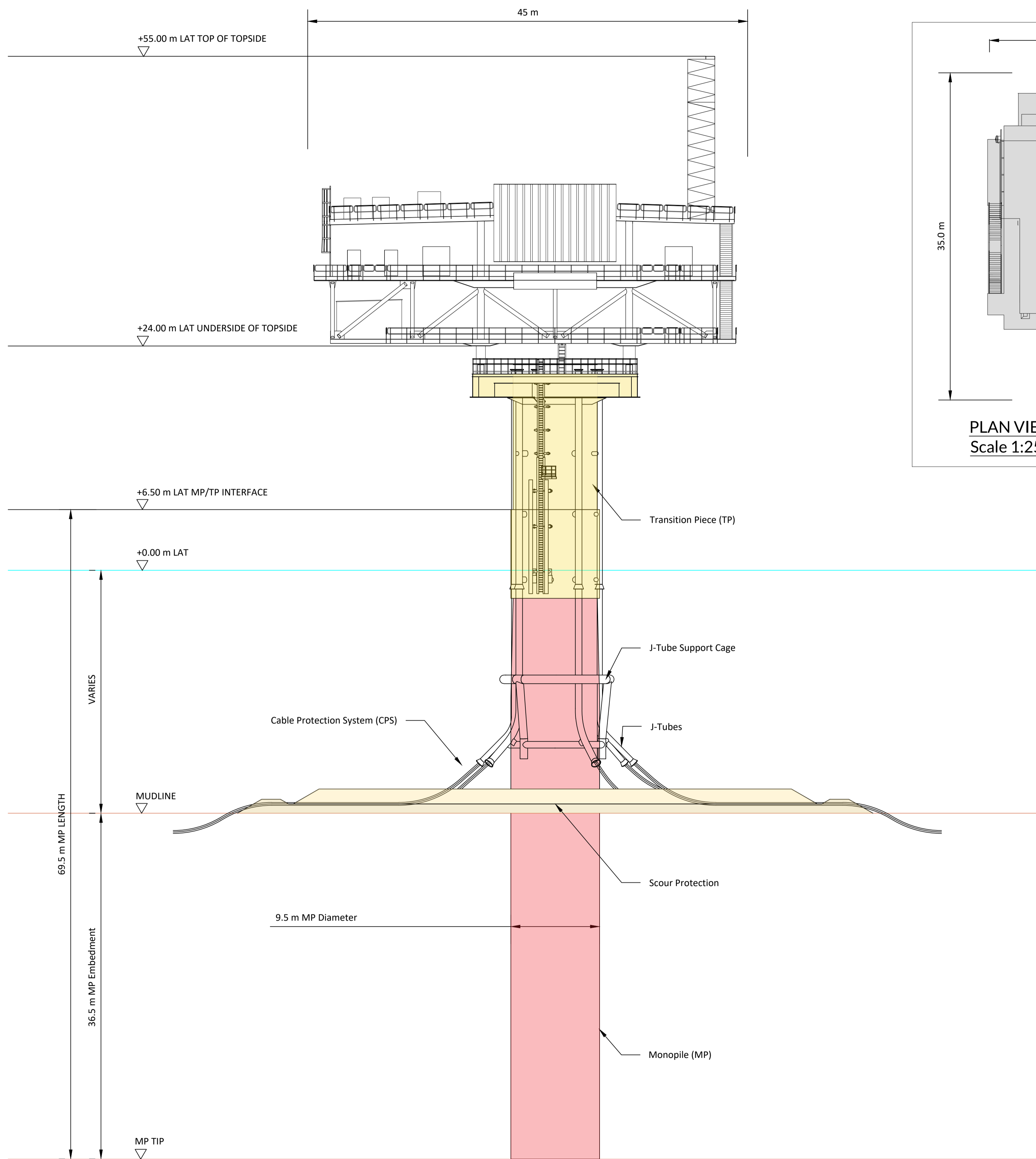
ELEVATION A Scale 1:250
