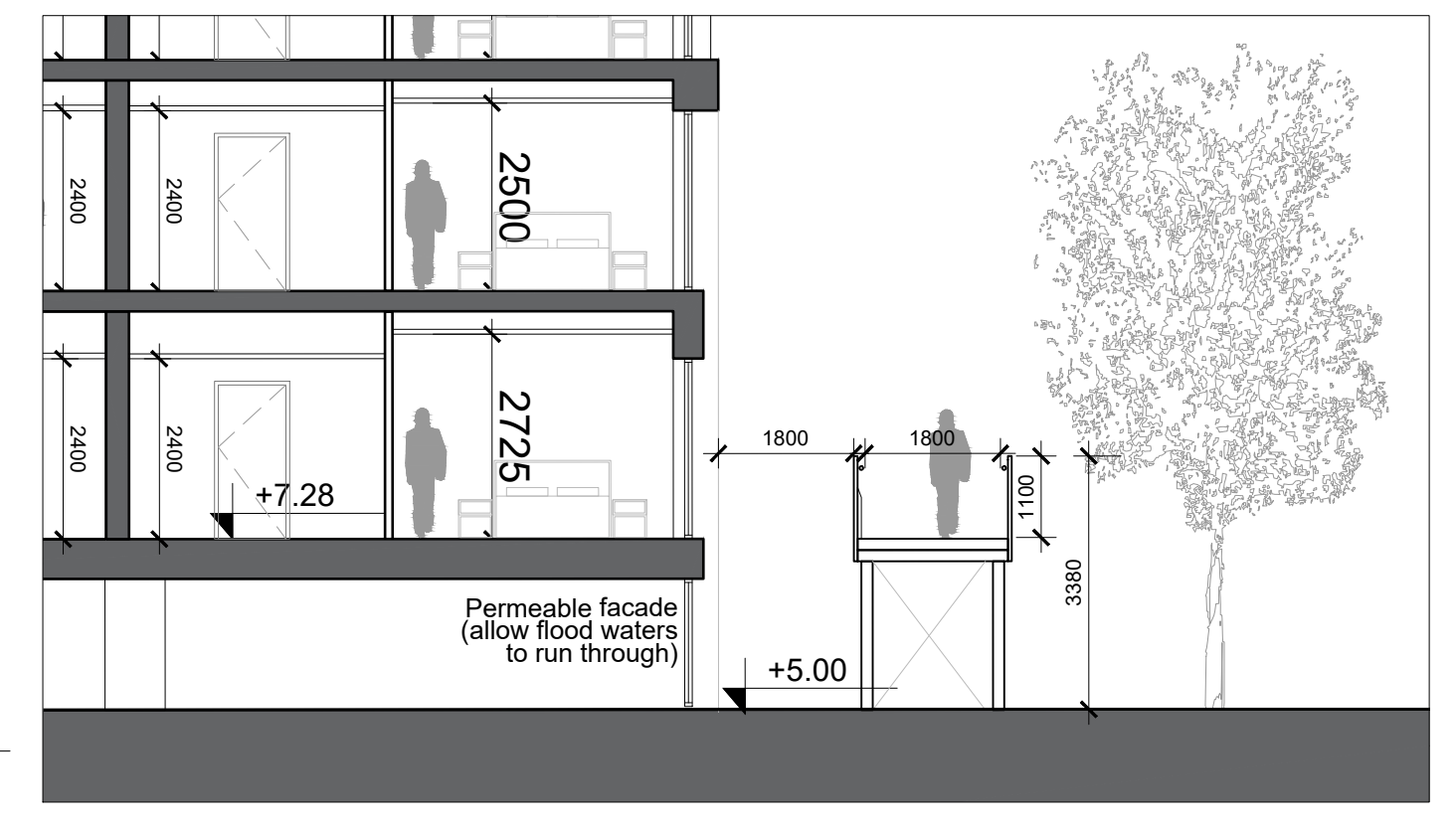
04 DETAIL SECTION 0422 1:100 @A1
