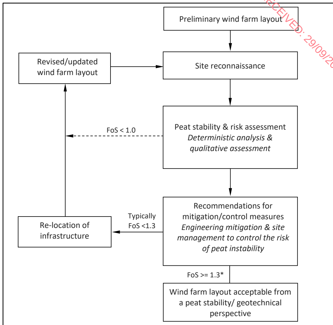
Figure 2.1: Methodology for Peat Stability Assessment
