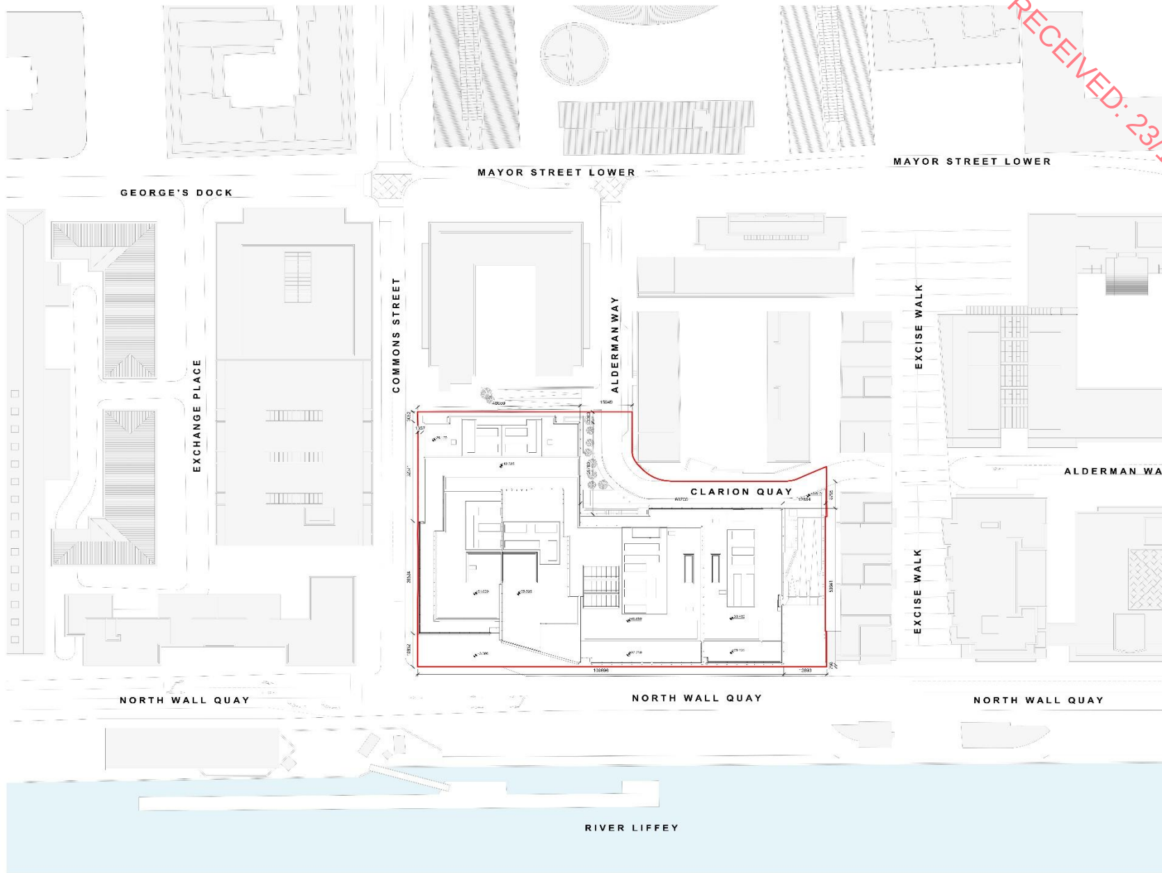
Figure 3. Proposed site plan
