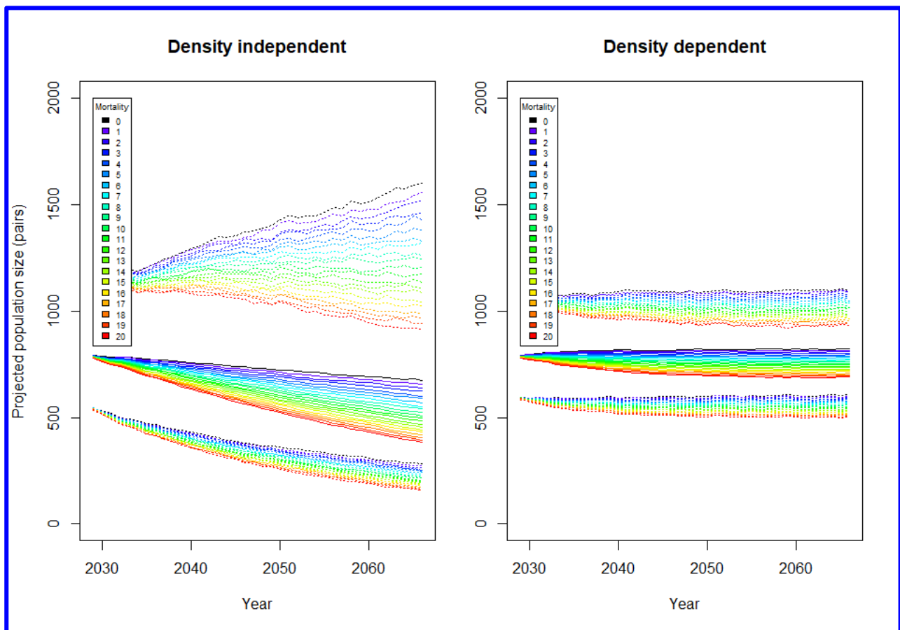
Figure 12.10.3: Density independent (left) and density dependent (right) population simulations for baseline (no impact) and adult mortality up to 20. Solid lines are the median from 5,000 simulations and the dashed lines are the 95% confidence intervals. Average productivity was 0.582, estimated using data from 2020-2024.
