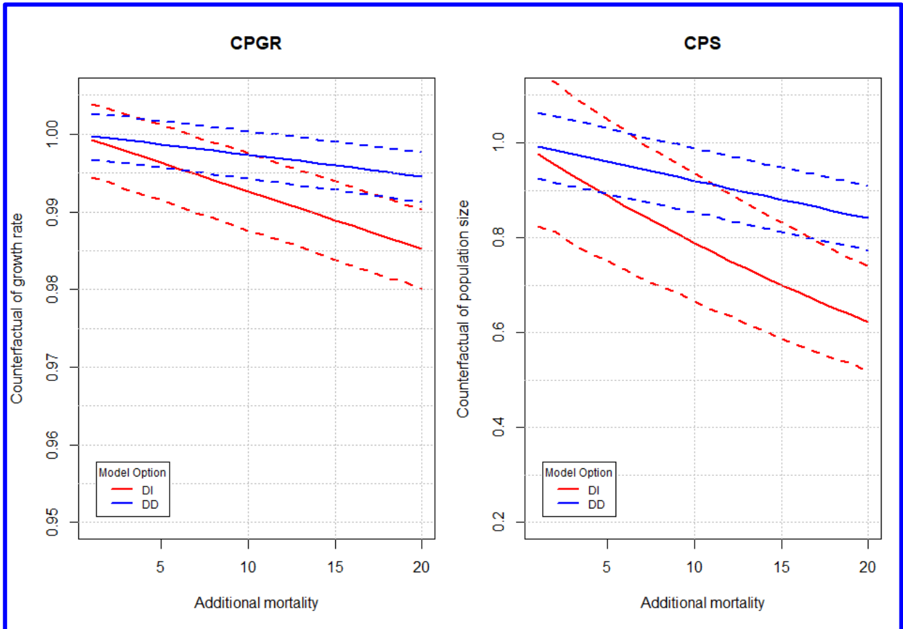
Figure 12.10.5: Median and 95% confidence intervals for the counterfactuals of population growth rate (CPGR; left) and population size (CPS; right) for the density independent (DI, red lines) and density dependent (DD, blue lines) simulations. Note the different scales on the y-axes, with a much wider range required for CPS. Average productivity was 0.582, estimated using data from 2020-2024.
