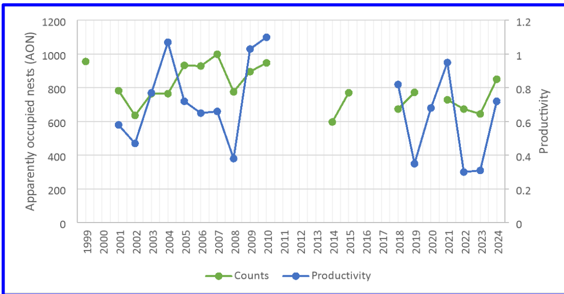
Figure 12.10.1: Wicklow Head kittiwake population data, 1999-2023/1999-2024.
