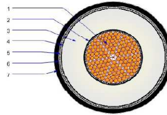
Figure 20: Typical crosssection of XLPE power cable (Diameter: 140mm; Weight: 40kg per meter).
