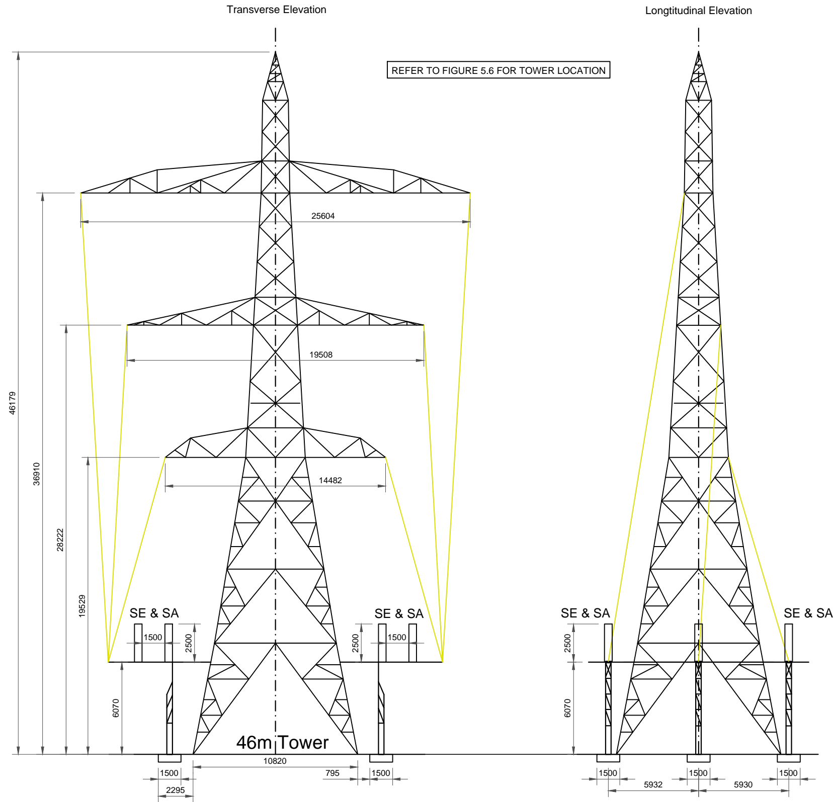
46m Tower Details
