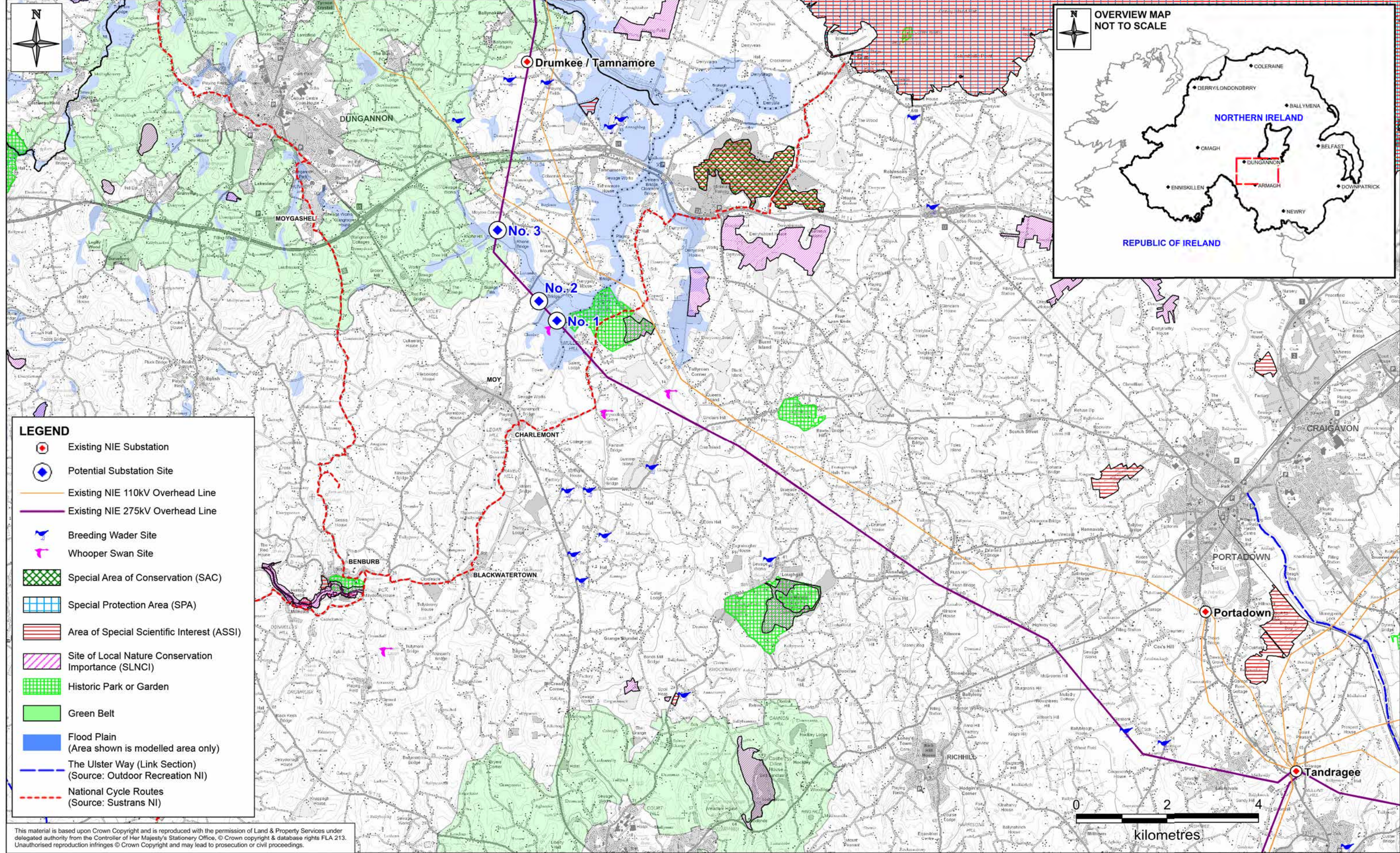
Title: FIGURE 4.5: SUBSTATION SITE ALTERNATIVES
