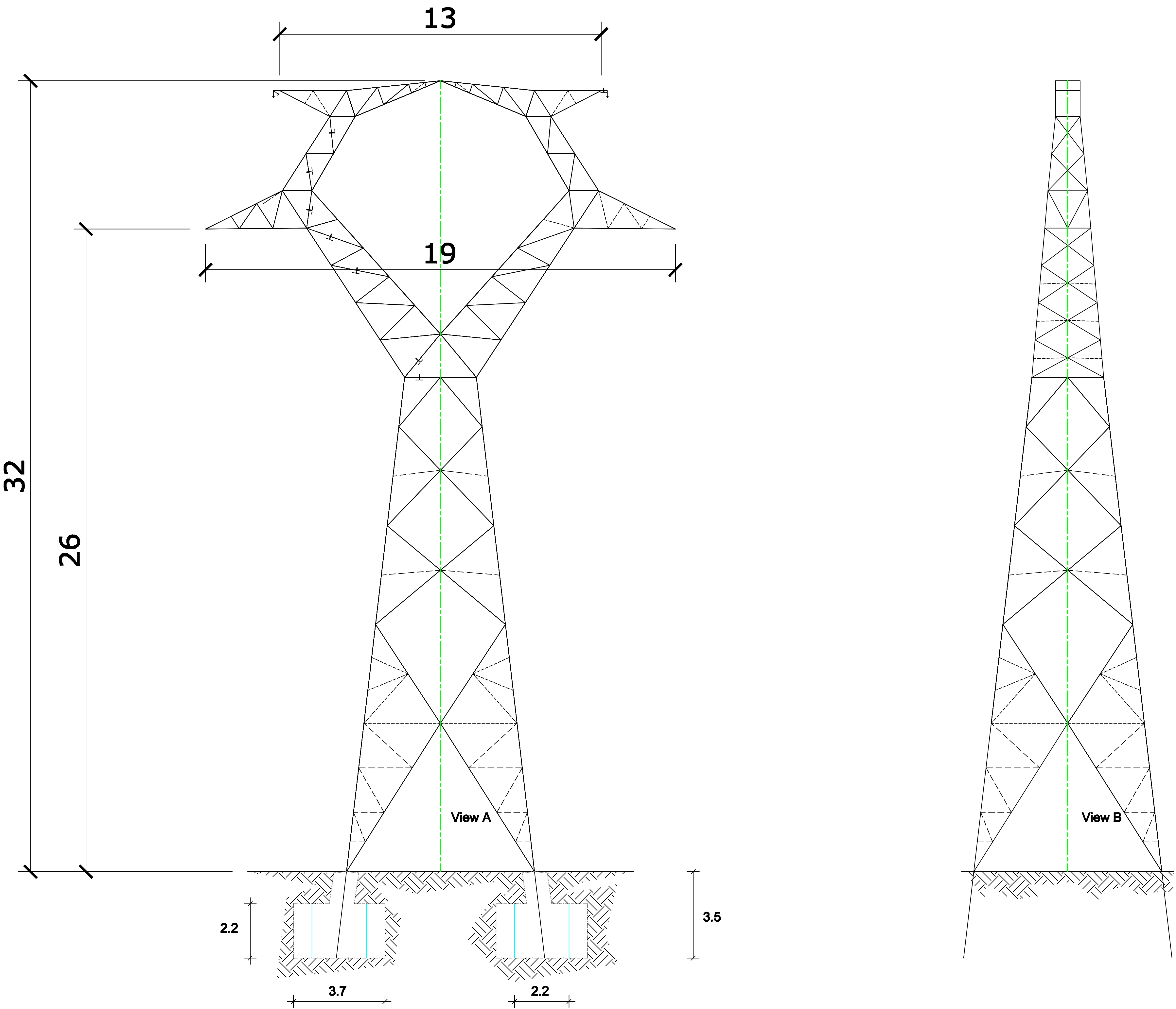
TITLE: TYPE " C-IV-1 " SUSPENSION TOWER TOWER OUTLINE JOB DESCRIPTION: 400 kV SINGLE CIRCUIT TRANSMISSION LINE TYRONE - CAVAN 400 kV LINE
