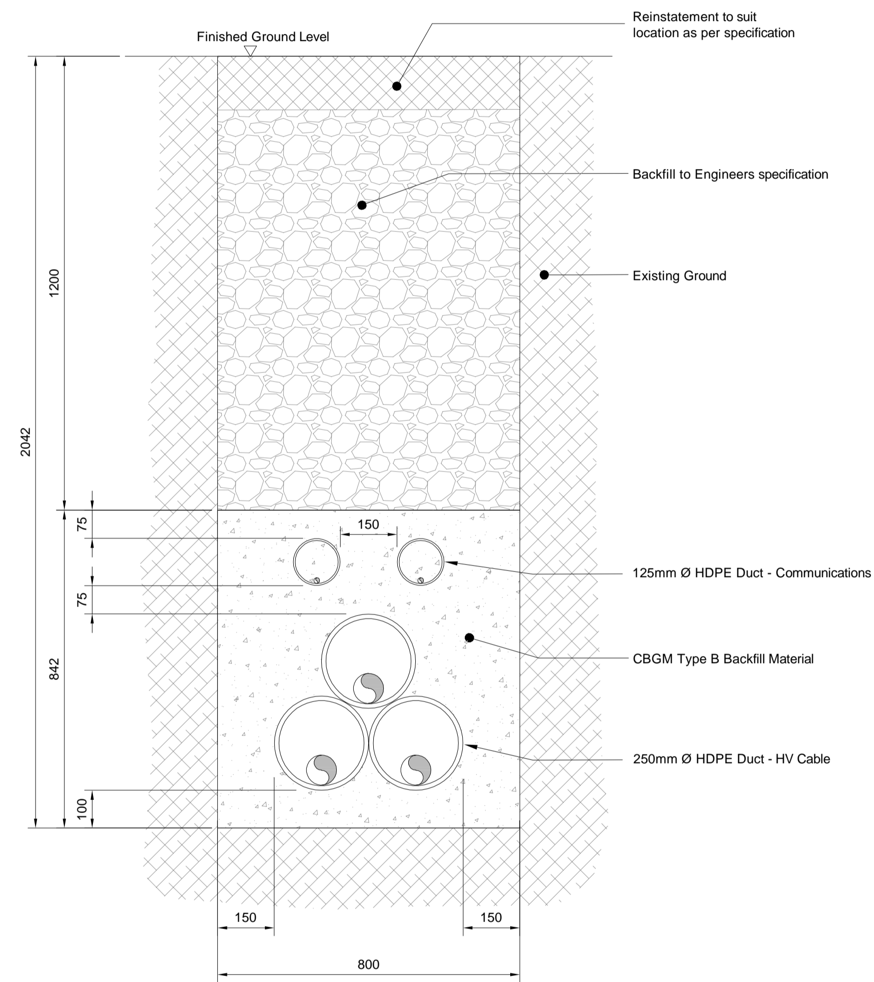
AC Cable - Typical Off-Road Section 1:10
