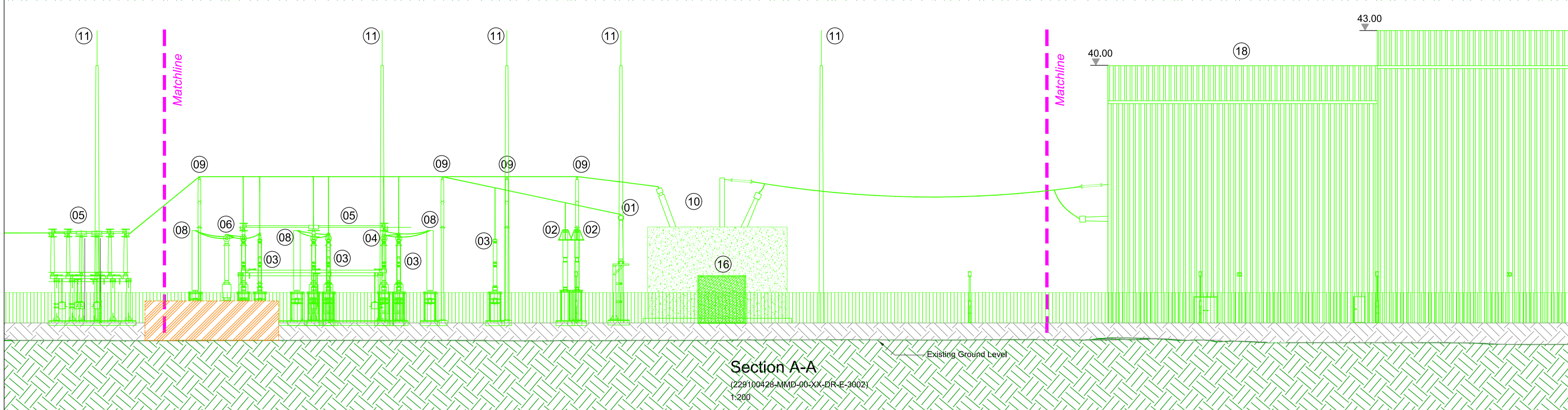
Section A-A (229100428-MMD-00-XX-DR-E-3002) 1:200
