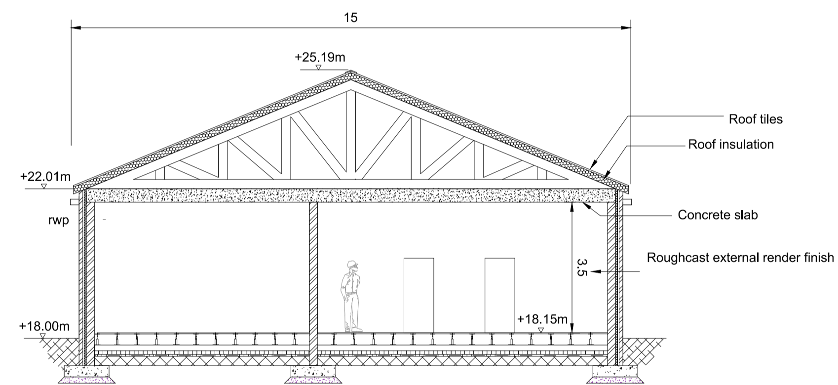
Section A 1:100
