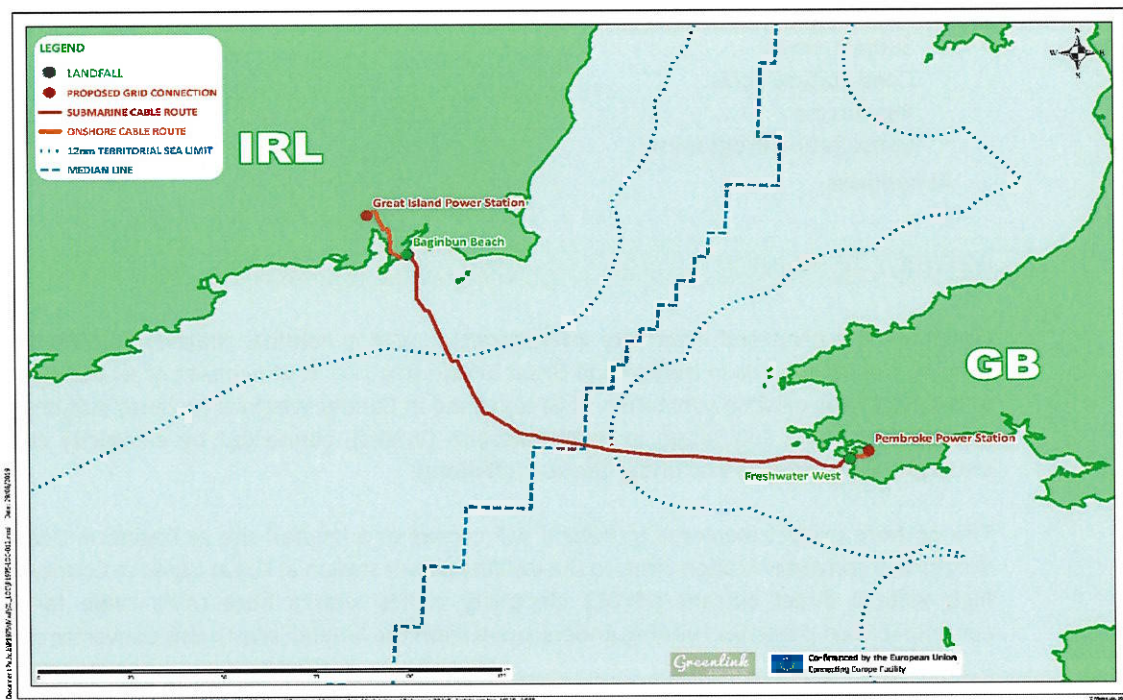
Figure 1-1 Greenlink Overview
