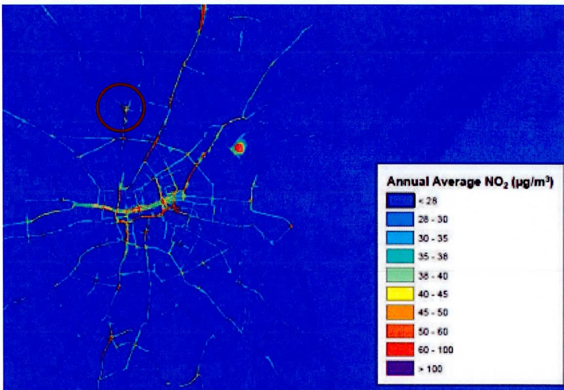
Modelled annual average NO 2 concentrations for 2015 in Dublin
